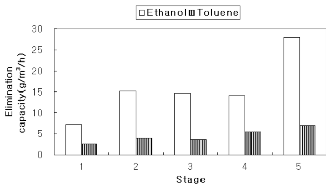
Fig. 17. Elimination capacity ( \text{g/m}^3/\text{h} ) of photo-catalytic reactor for simultaneous treatment of ethanol and toluene at each stage.
