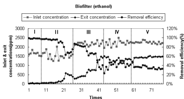
Fig. 13b. Removal efficiency, inlet and exit concentrations of biofilter system without photo-catalytic reactor versus times [Lim and Park, 2005].
